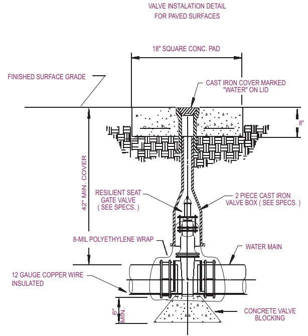
VALVE INSTALLATION DETAIL SEE PW04
