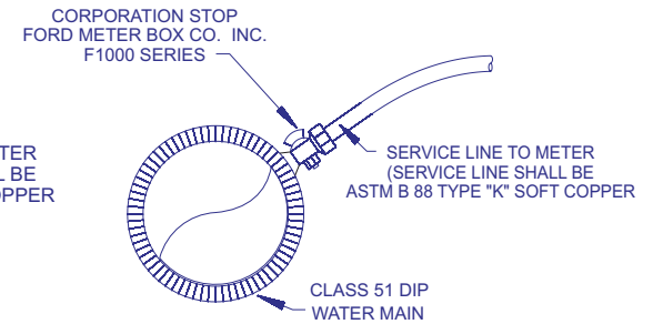
SERVICE TAP DETAIL DUCTILE IRON AND CAST IRON PIPE "NON POLY WRAP"
