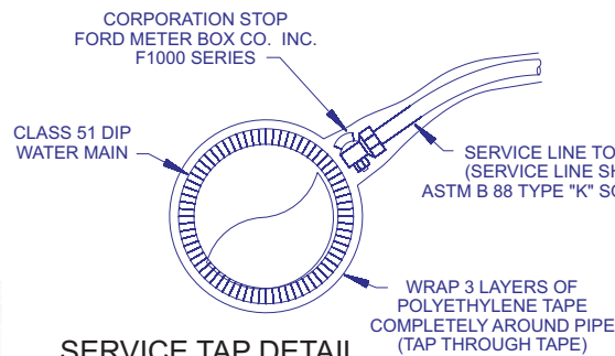
SERVICE TAP DETAIL DUCTILE IRON PIPE POLYETHYLENE ENCASED
